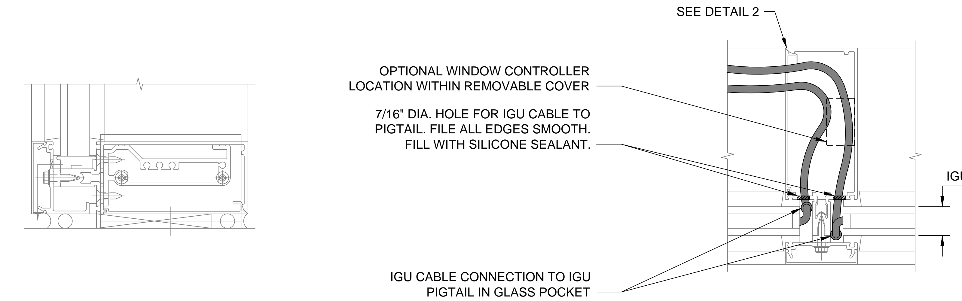
DETAIL 3 SILL
