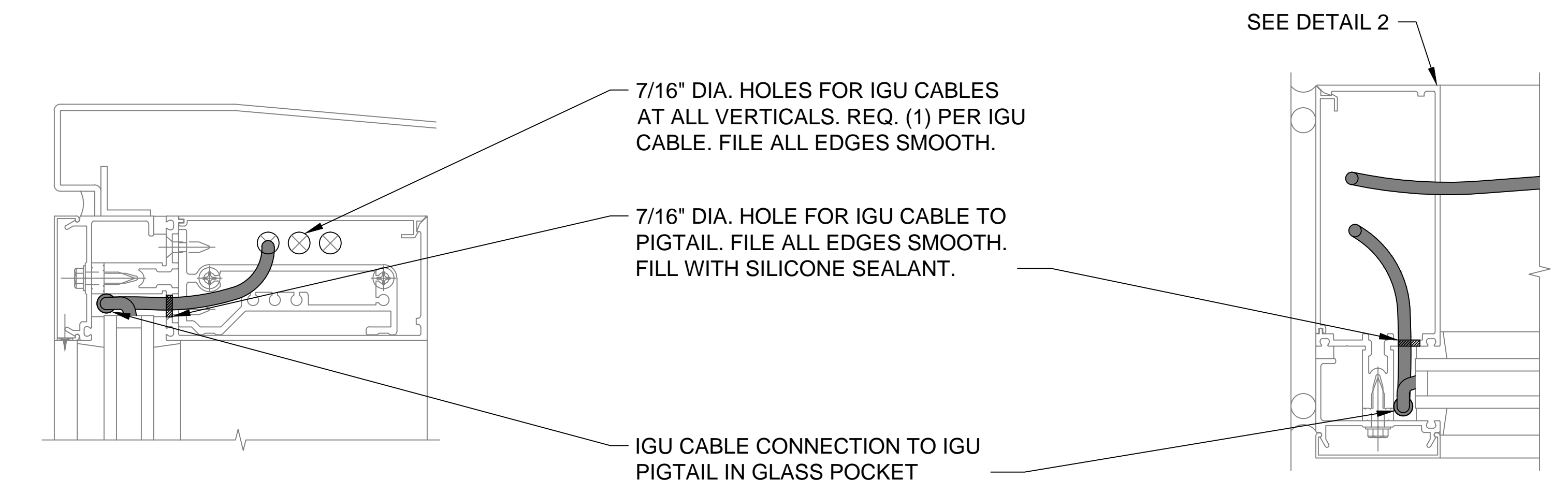
DETAIL 1 HEAD
