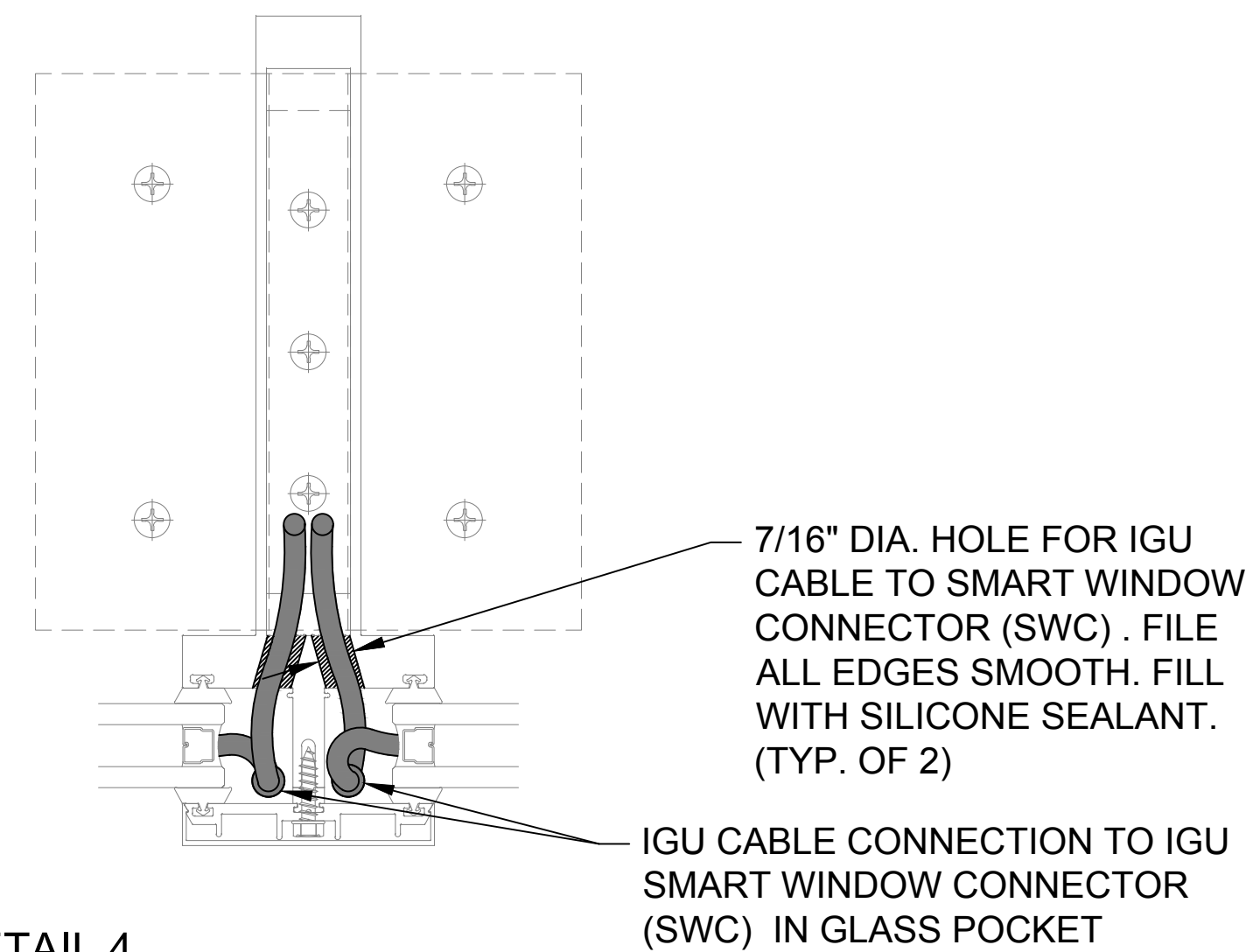
DETAIL 4 VERTICAL MULLION, CAPTURED GLAZING
