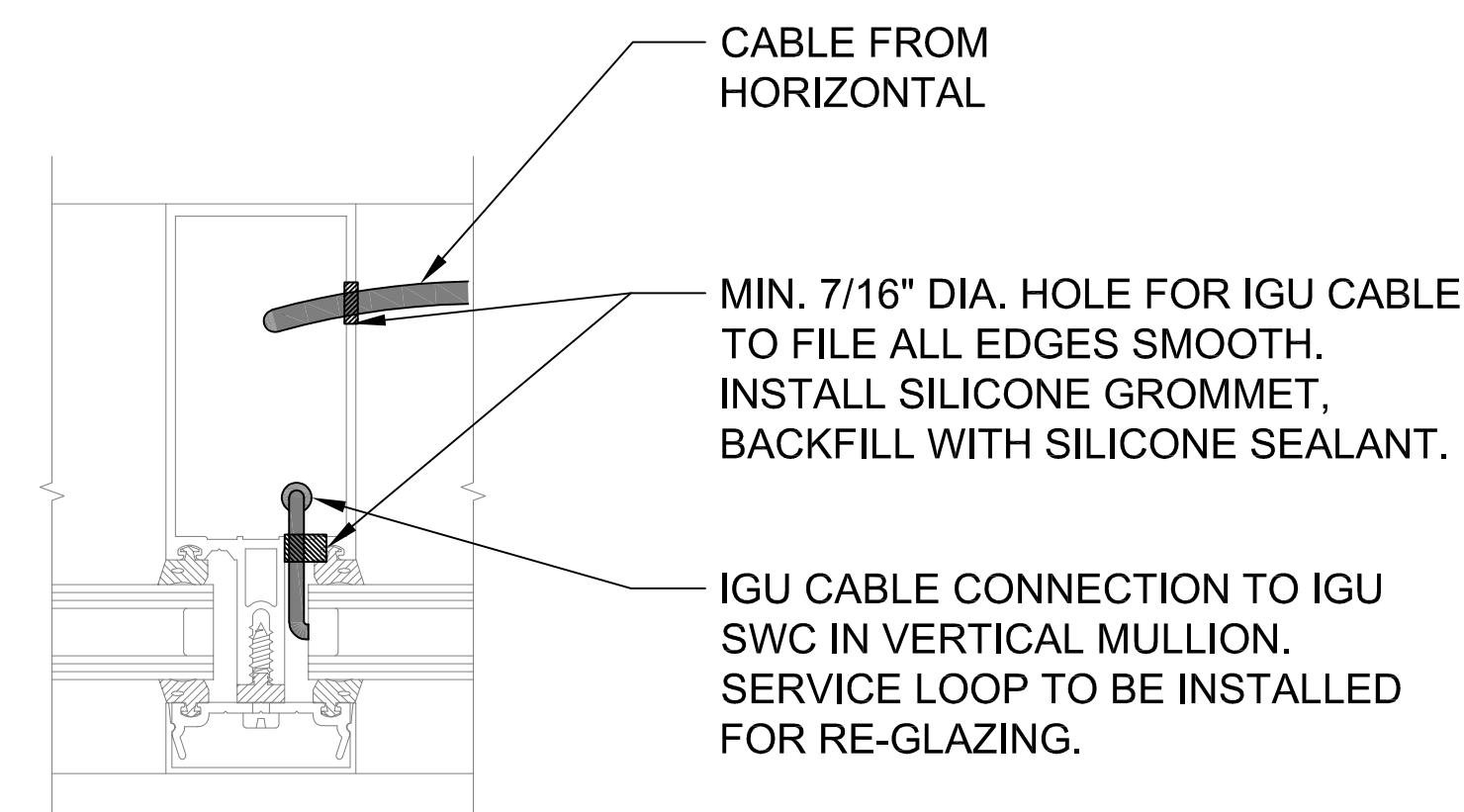
DETAIL 5 VERTICAL MULLION
