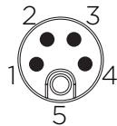
Male Pin Assignment
